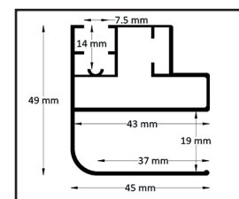
Corner profile
