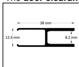
Fixed-side glass profile
