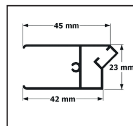
Magnet profile
