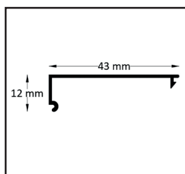
Wall profile cover
