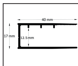
Fixed-side wall profile
