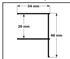
Profile wall
