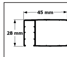
Corner profile
