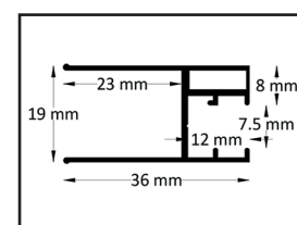
Fixed glass profile
