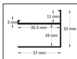
Fixed wall profile
