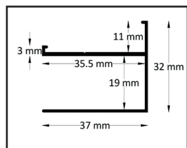
Fixed wall profile
