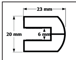
Glass profile
