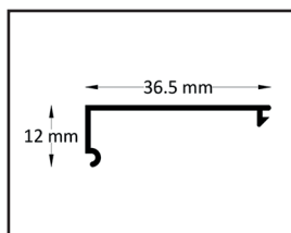
Wall profile cover
