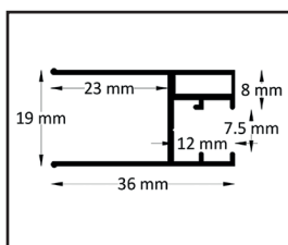
Fixed glass profile
