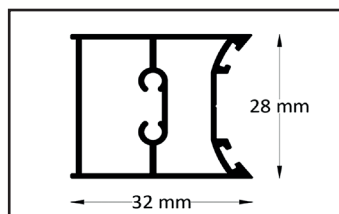
Hinge profile
