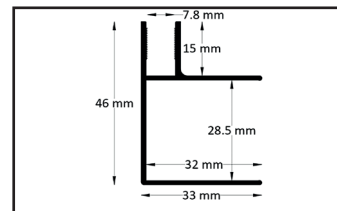
Corner profile
