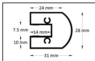
Glass rotating profile
