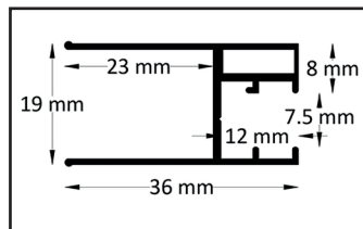
Fixed glass profile
