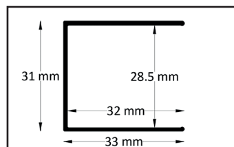
Door-side wall profile
