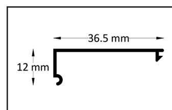
Wall profile cover
