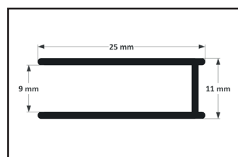
Door closure profile
