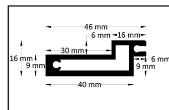
Wheel slide bar
