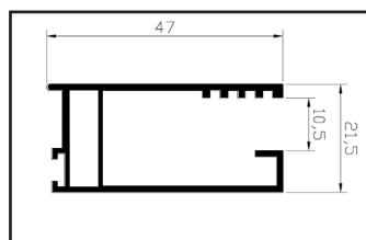
Wall profile fixed side
