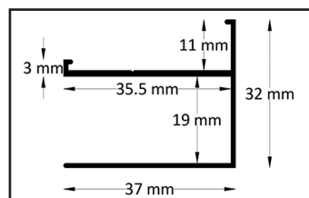
Profile wall
