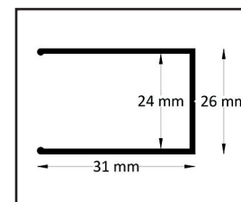
Fixed glass wall profile
