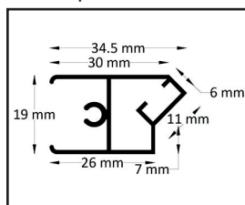
Magnet striker profile
