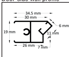
Magnet striker profile
