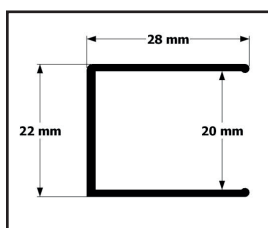
Door-side wall profile
