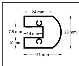
Rotating glass profile
