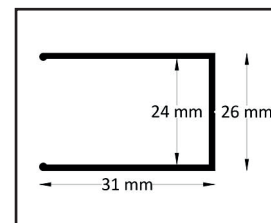
Fixed glass wall profile
