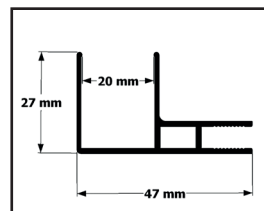
Angular profile
