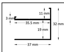
Fixed wall profile
