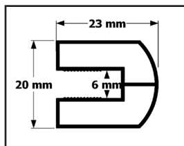
Glass profile
