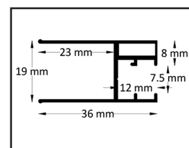
Fixed glass profile
