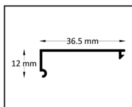
Wall profile cover
