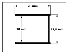
Wall profile
