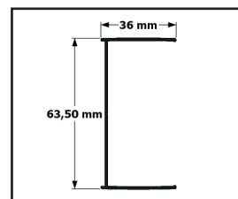
Profile wall
