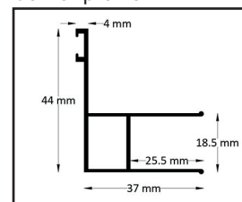
Door closure profile
