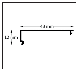
Fixed wall glass profile
