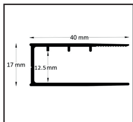
Fixed wall profile
