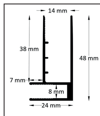
Corner profile
