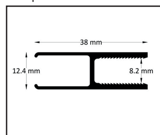
Glass profile
