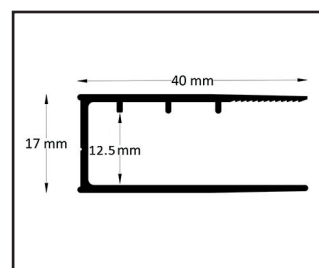
Wall profile
