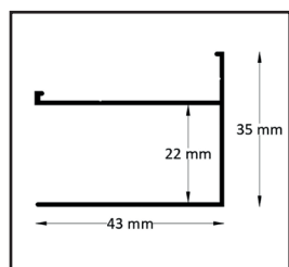
Wall profile
