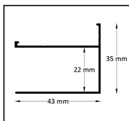
Wall profile
