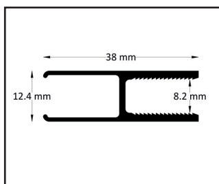
Profile glass
