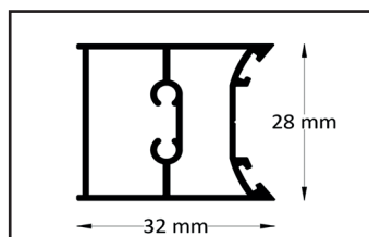
Hinge profile
