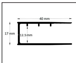
Profile wall
