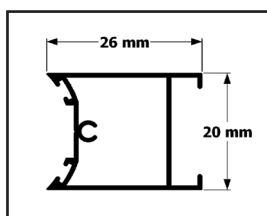
Hinge profile
