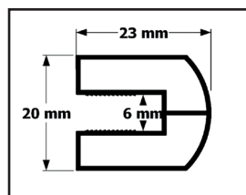
Glass profile
