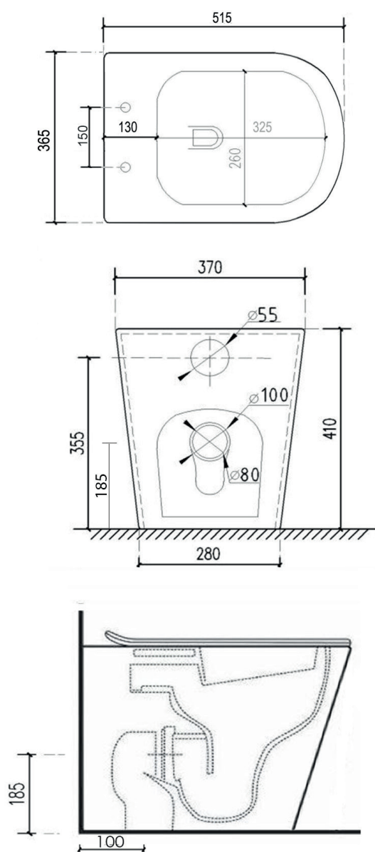
TOILET (art.GIO.42)
