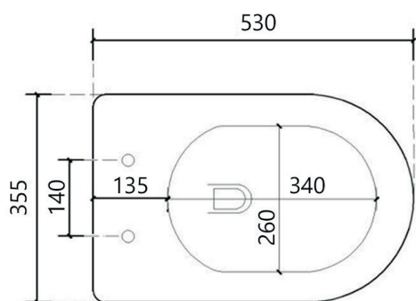
TOILET (art.GIO.26RIM)
