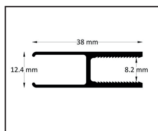
Glass profile
